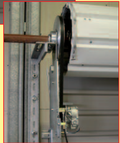
815-SL SLIM-LINE operator to suit applications with limited clearance
