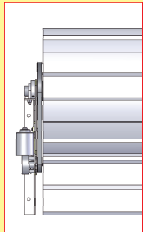
815-SD STANDARD operator
